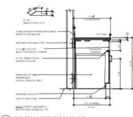
TYP. TRASH/RECYCLE BASE UNIT 1/4" = 1'-0"
