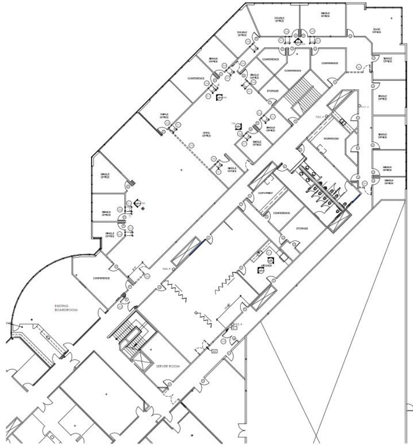
DEMOLITION AND PARTITION PLAN SCALE: 1/8" = 1'-0"
