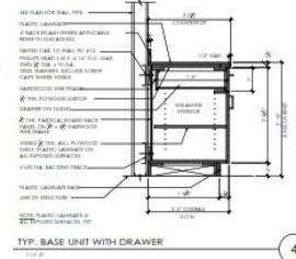
TYP. BASE UNIT WITH DRAWER 1/4" = 1'-0"
